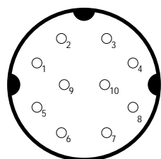
F90x/N90s connector front view
